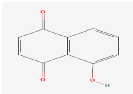
Figure 4. Chemical structure of Juglone ( C_{10}H_6O_3 ) (Salık & Çakmakçı, 2023)
