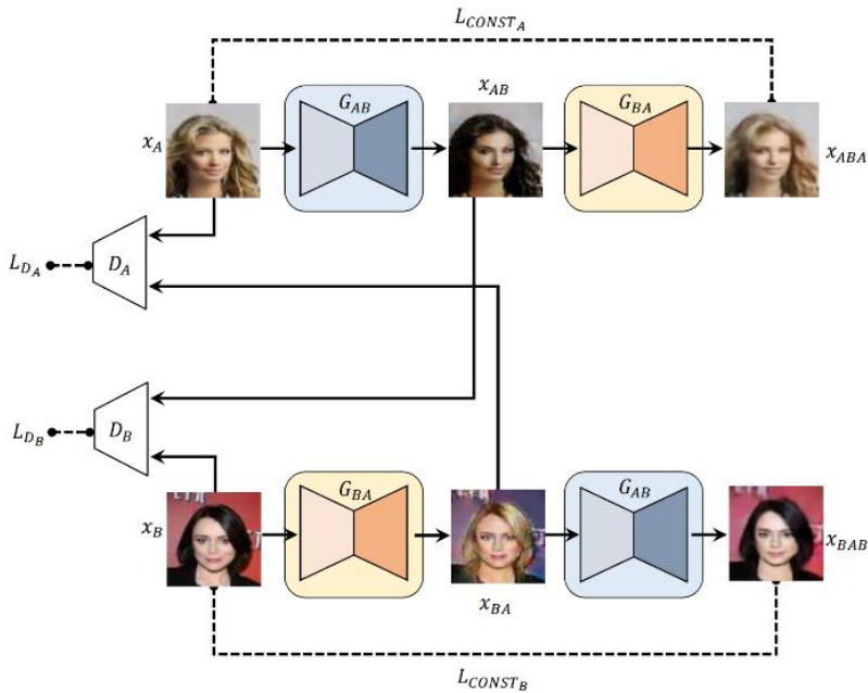
Figure 6. DiscoGAN Architecture Shown in Article (Kim et al. 2017)
