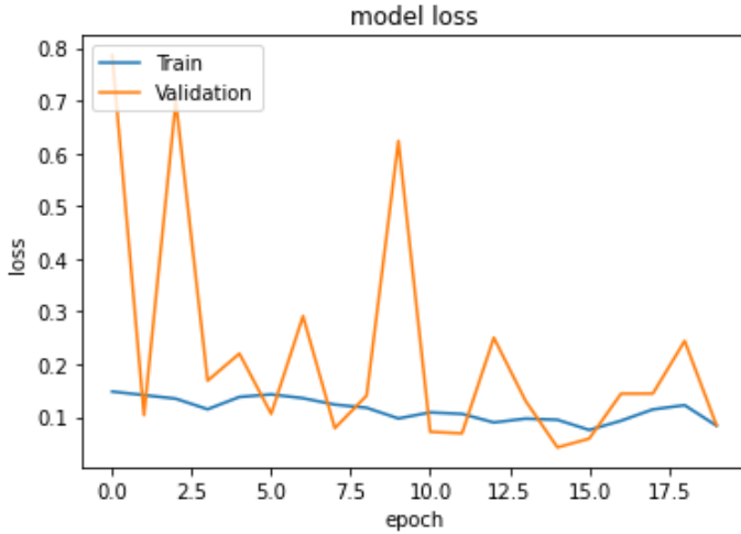
Figure 2. Model Loss
