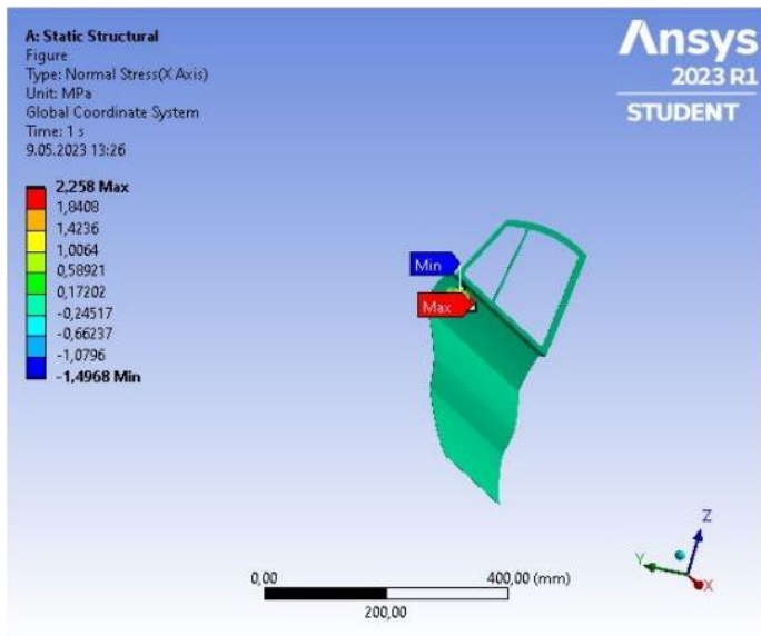
Figure 7. Normal Stress
