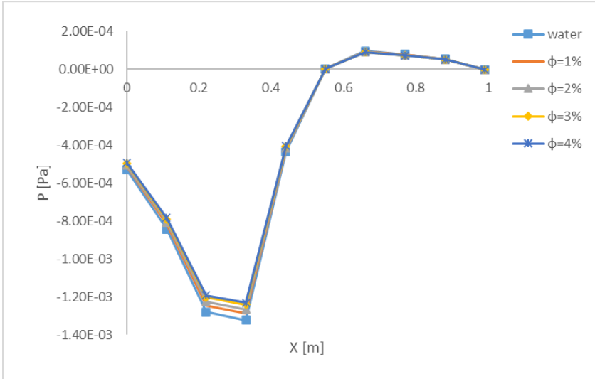
(a) Re = 500
