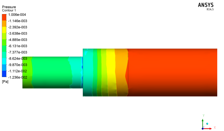
(b) 4% Nanofluid
