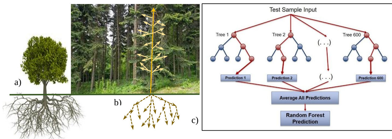
Figure 1. a) Consideration of a) individual tree, (Embark, 2023), and b) forest, might be the base concept of decision-systems here, c) random-forest decision reasoning is also applicable for the cases including complex and large numbered data conditions (Blakely, et al., 2018).
