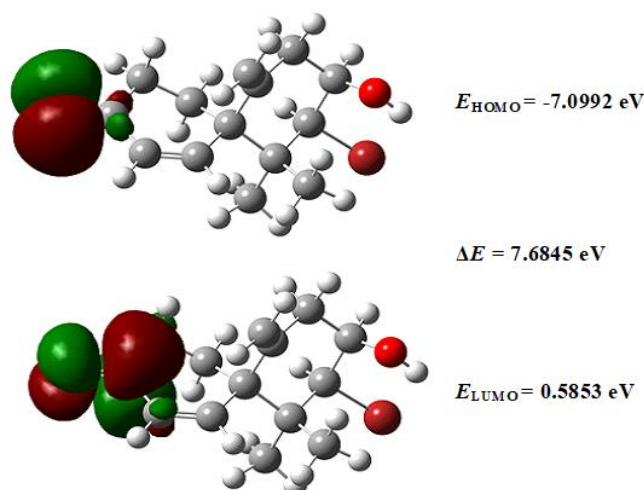
Figure 4. HOMO and LUMO Distributions
