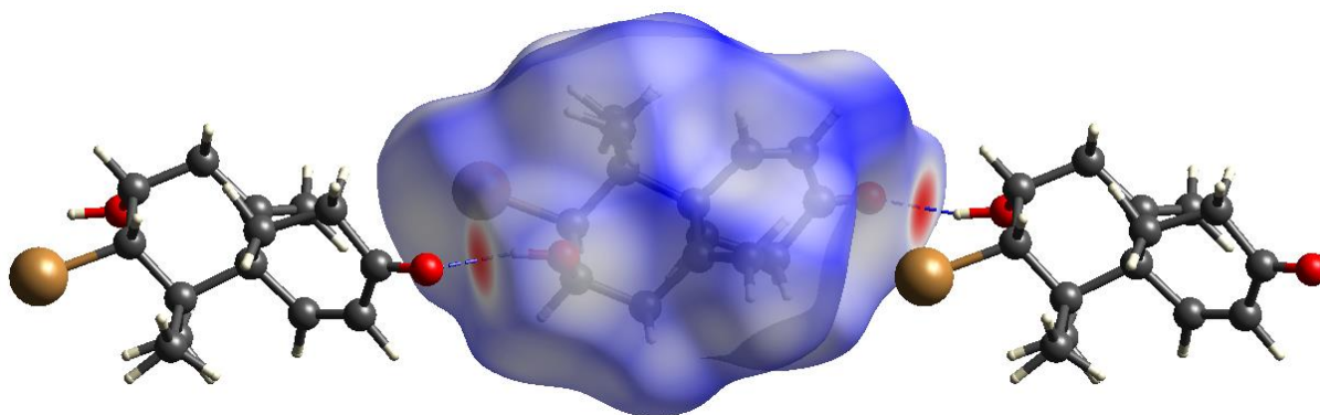
Figure 9. dnorm HS Map Illustrating the Intermolecular Contact Regions of the Investigated Molecule
