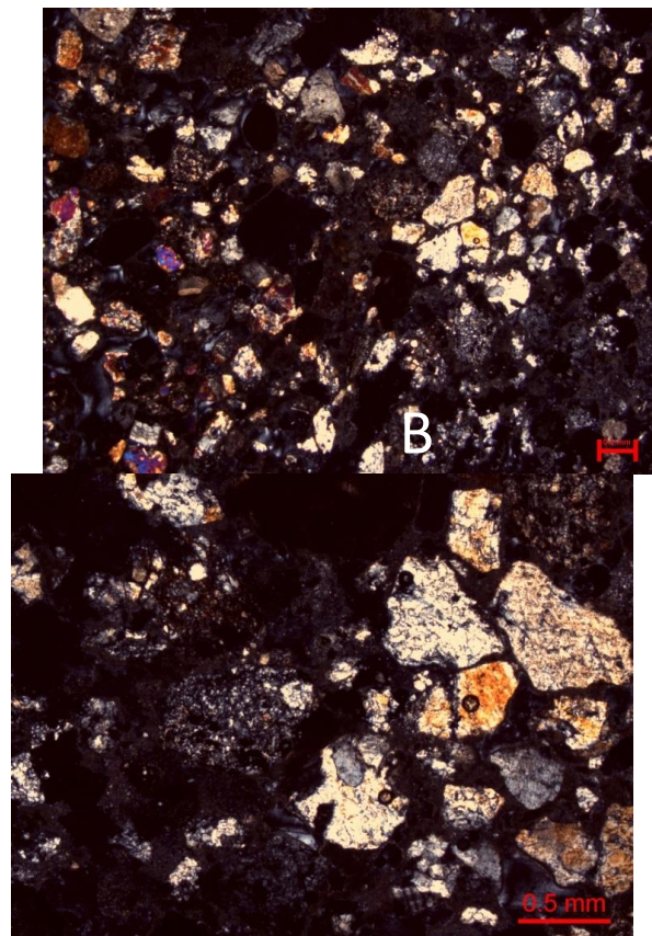
Figure 14. General view of thin section of Sample 4 under polarising microscope. A-B. The general texture of the sample and the aggregate and mineral particles in it (Double Nicol)
